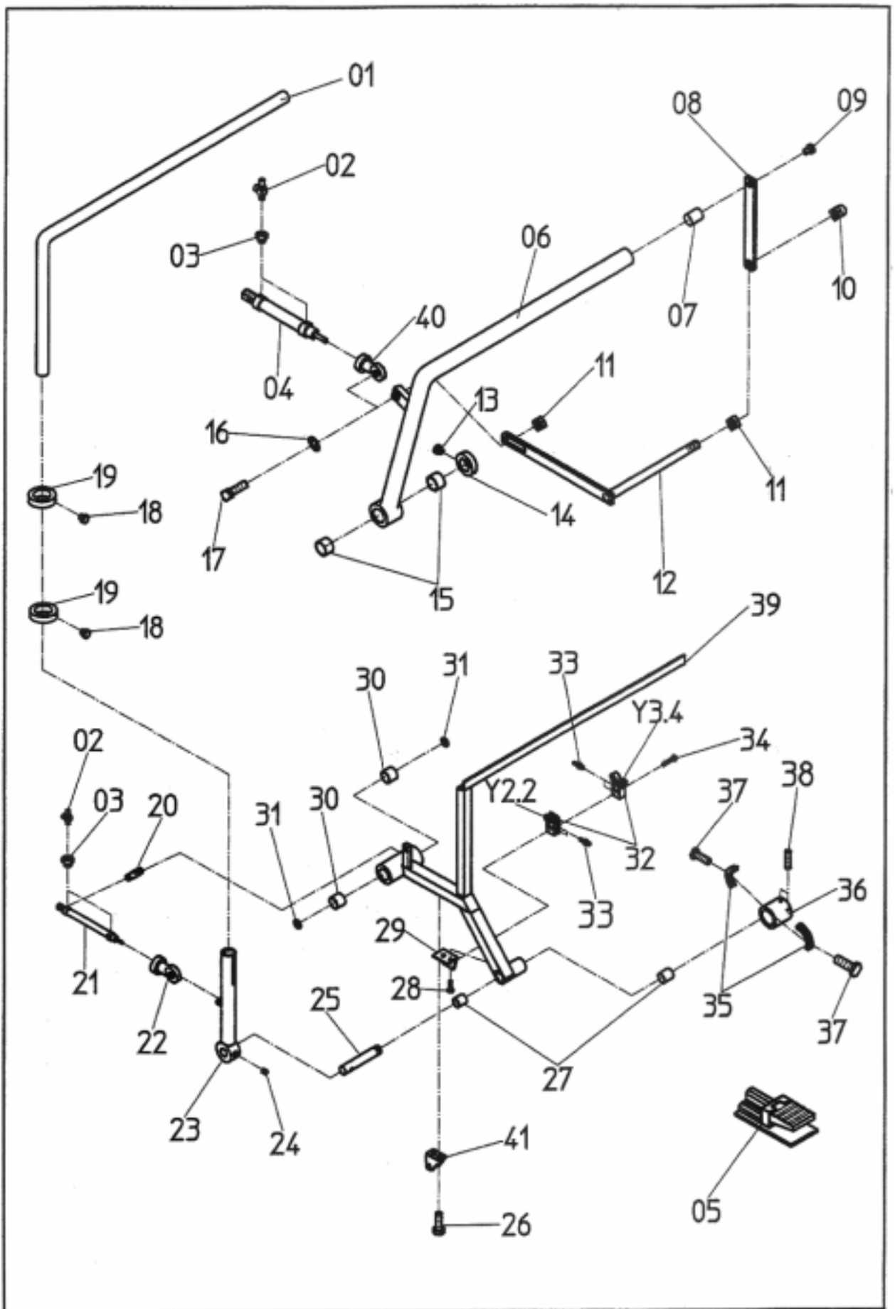
TAFEL 2 KLAPPSTAPLER 201/6
